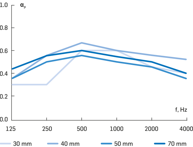
Suspension 200 mm
